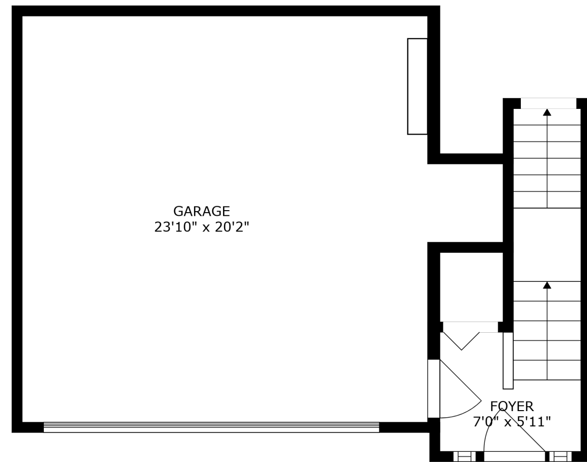
FLOOR 1
