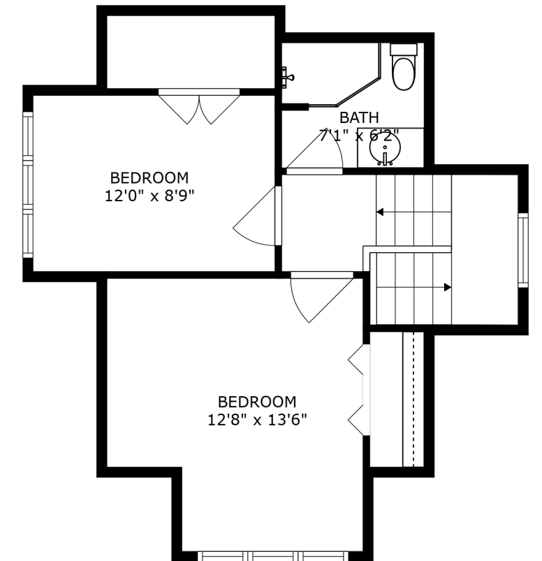
FLOOR 4
