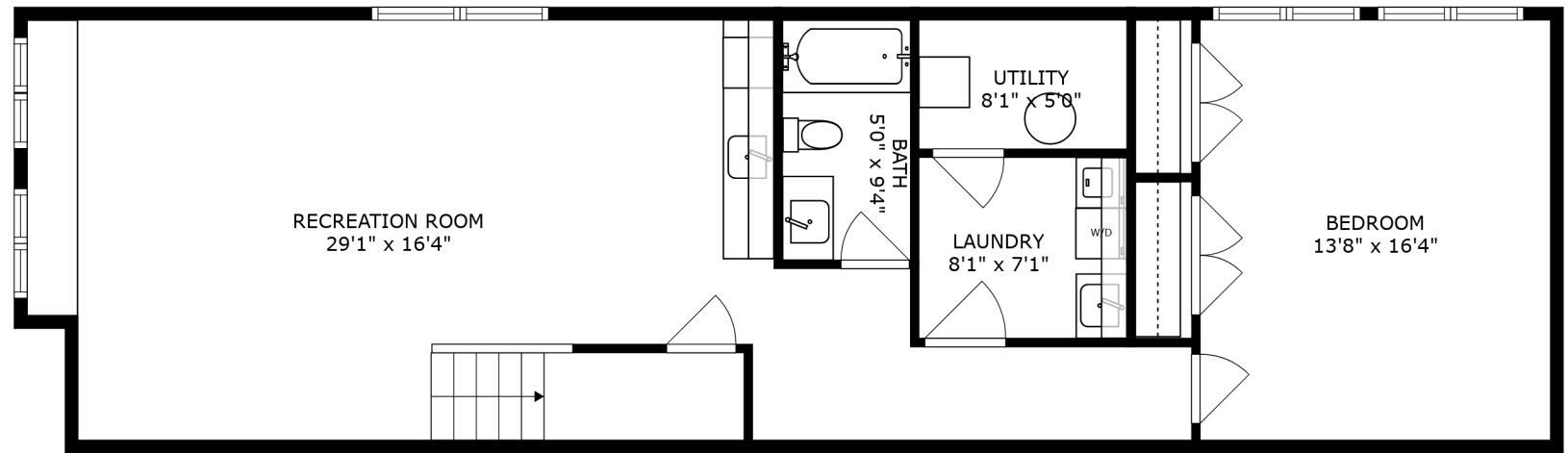
FLOOR 1
