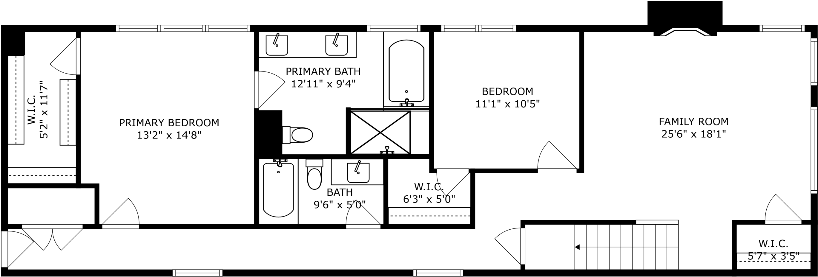
FLOOR 1
