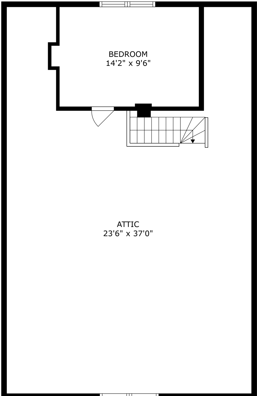
FLOOR 3
