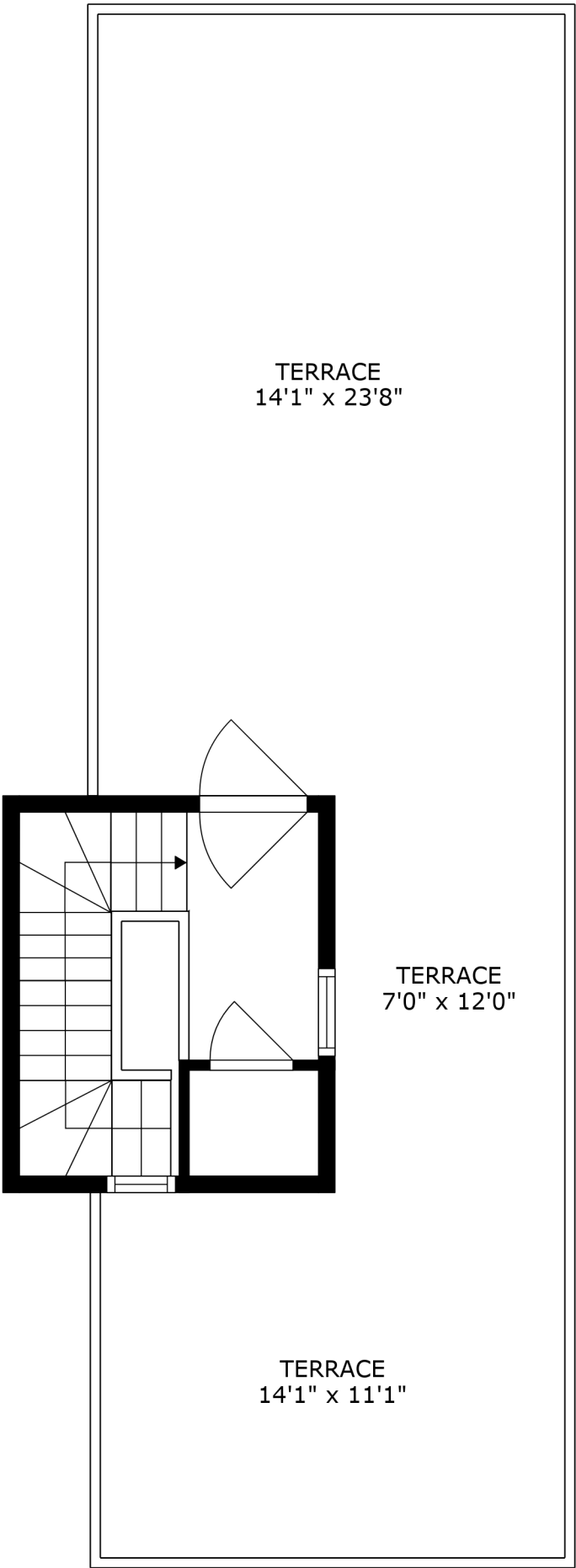
FLOOR 4
