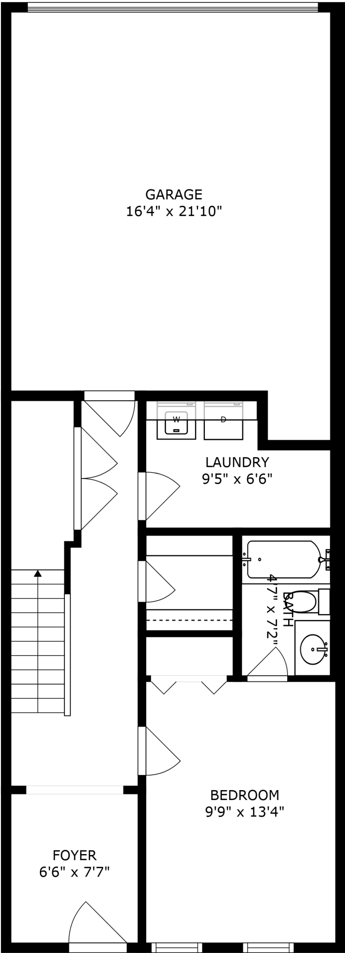
FLOOR 1
