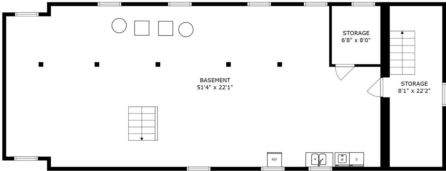
FLOOR 1
