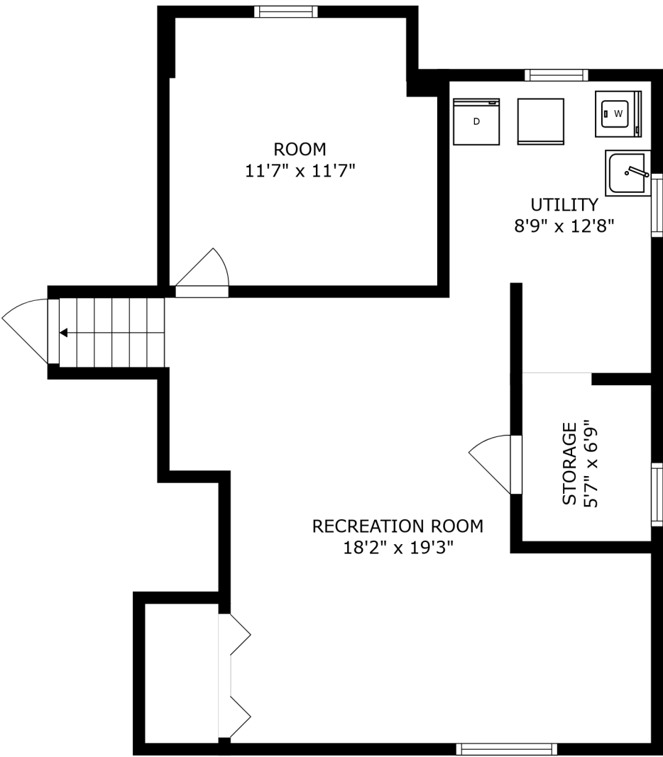
FLOOR 1
