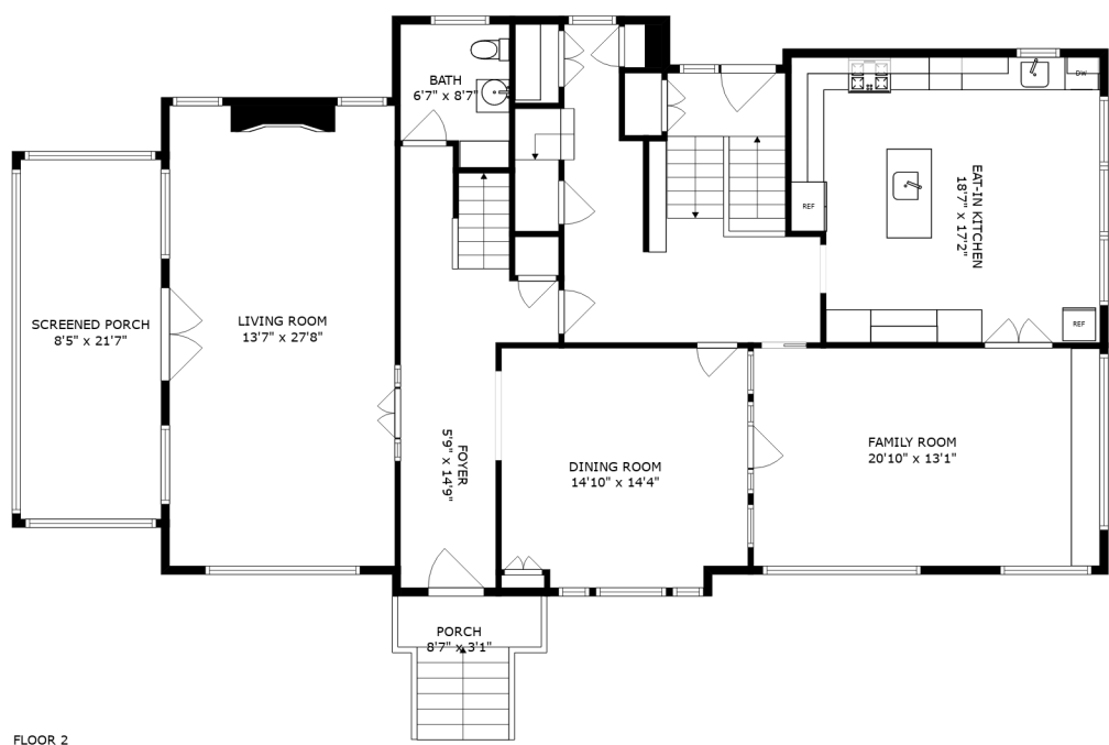
FLOOR 2
