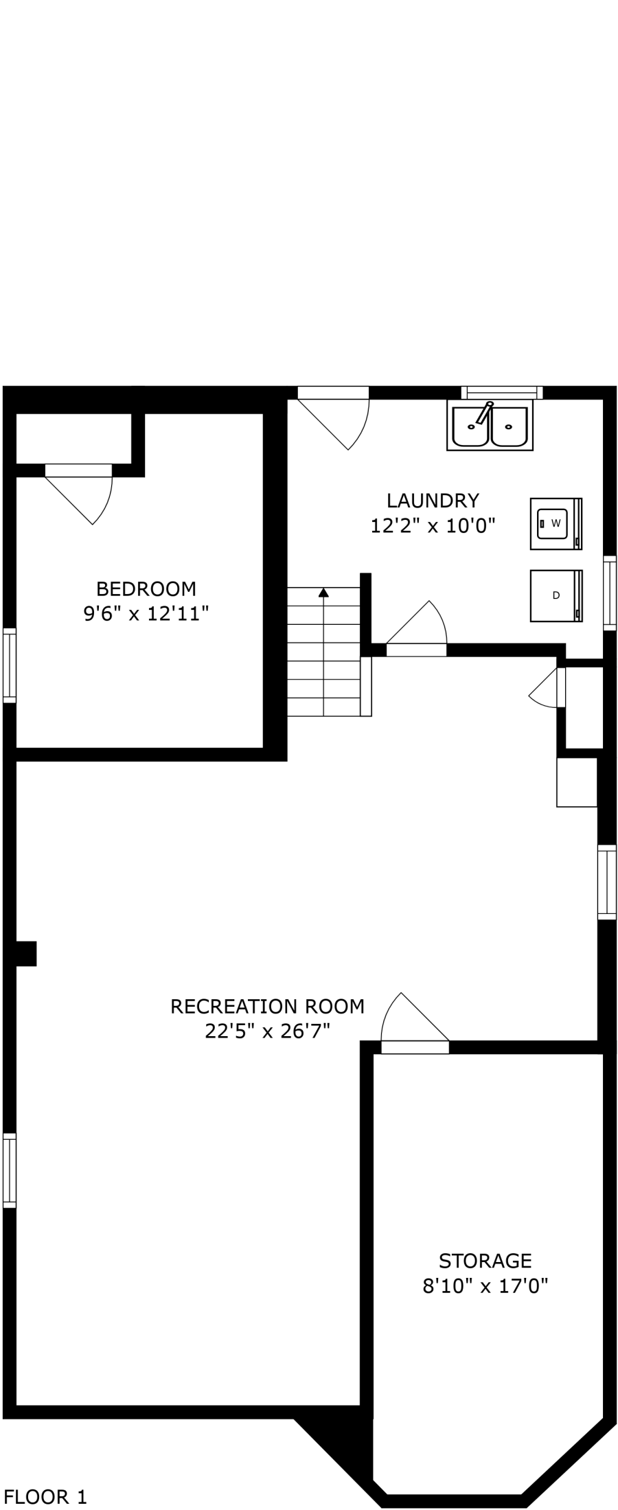
FLOOR 1
