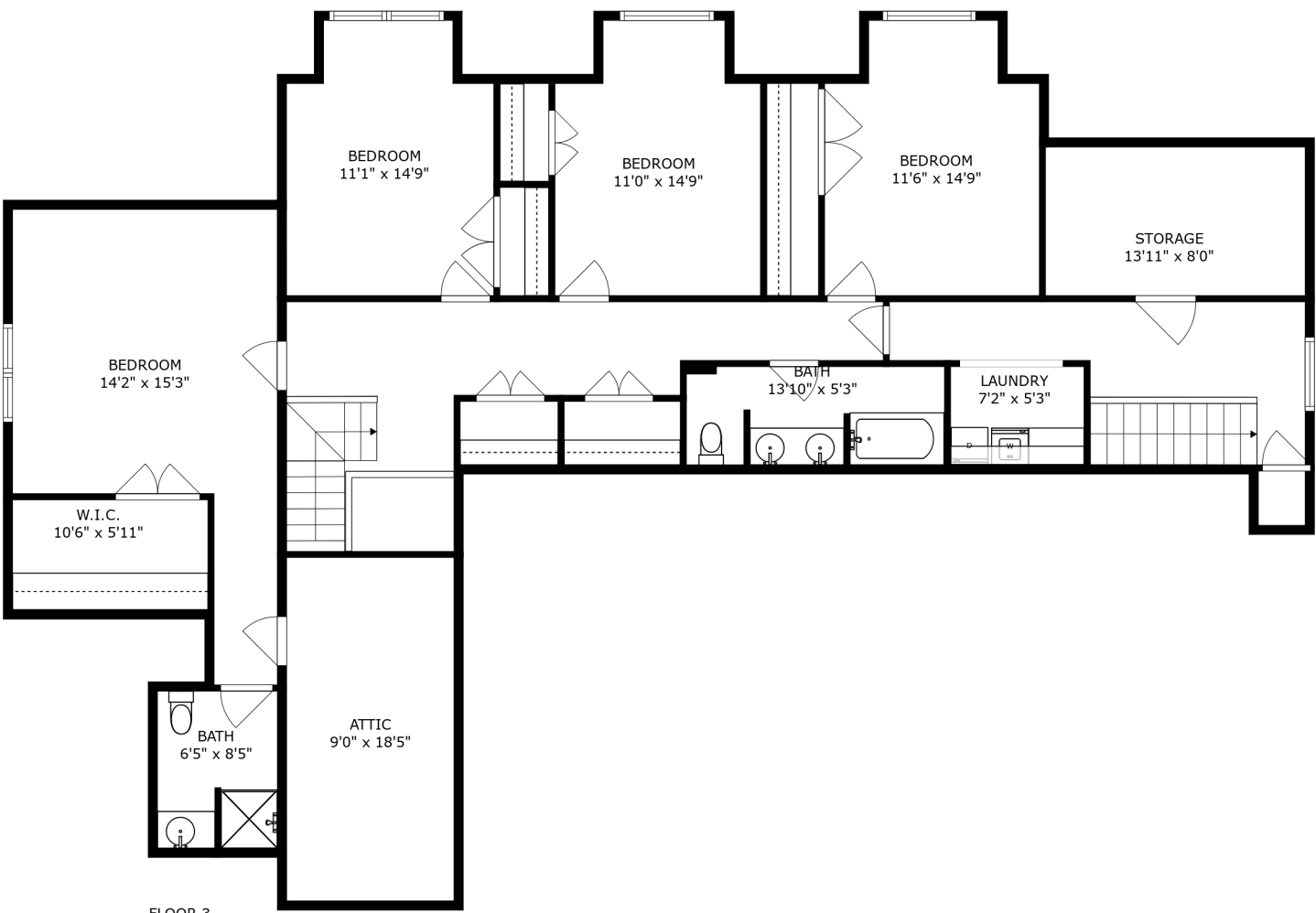
FLOOR 3
