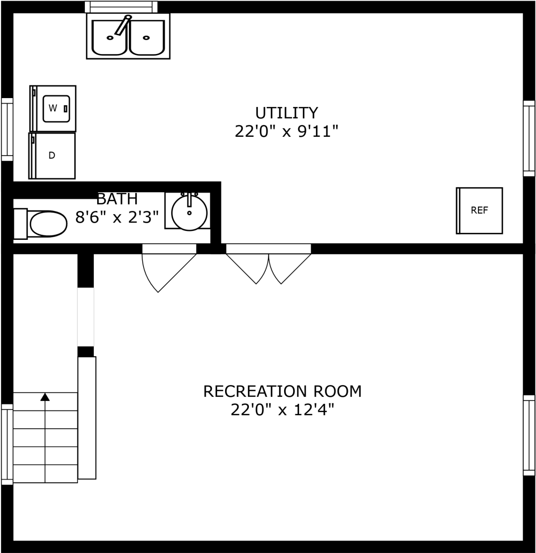
FLOOR 1
