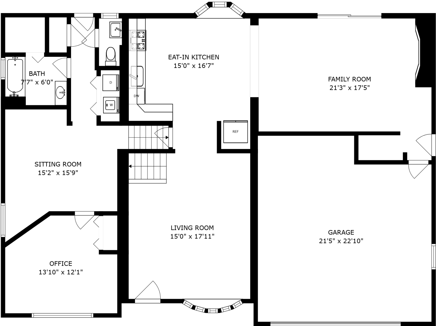
FLOOR 1
