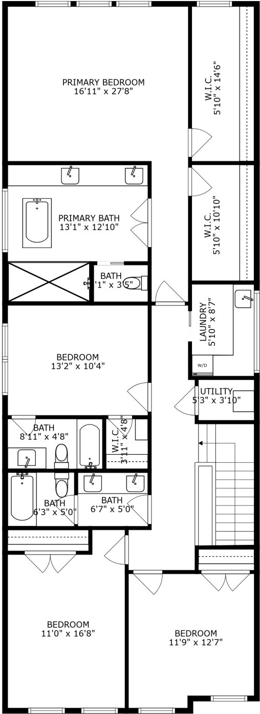
FLOOR 3
