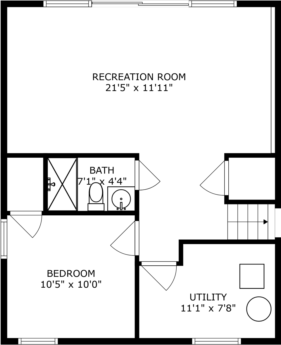
FLOOR 1
