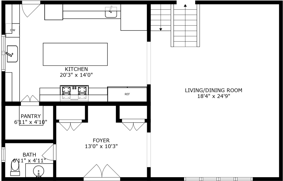
FLOOR 3
