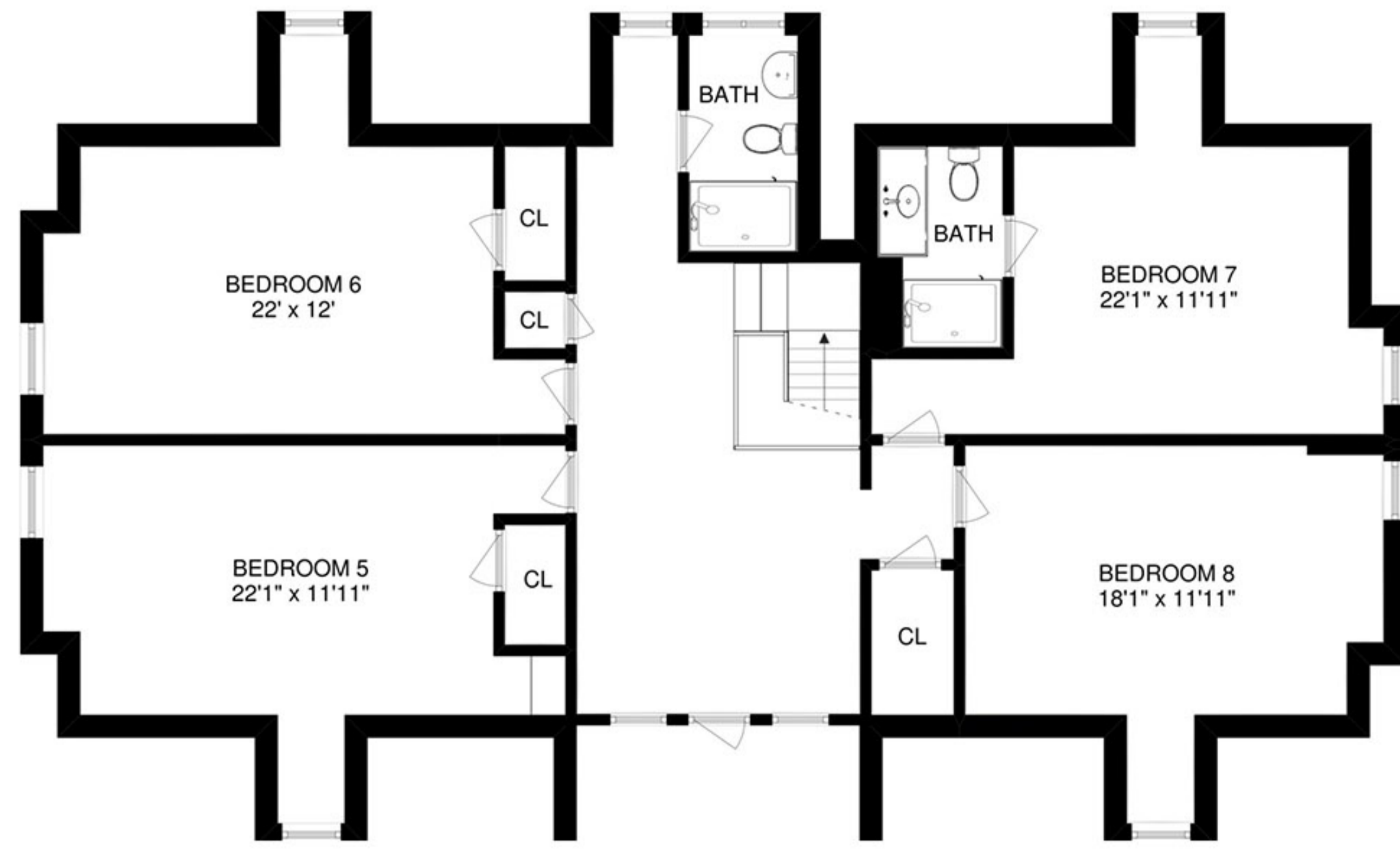
THIRD FLOOR
