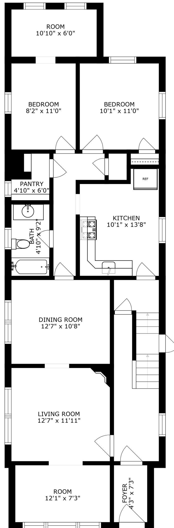
FLOOR 2
