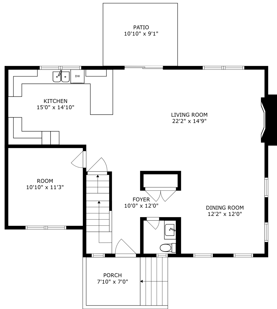
FLOOR 2
