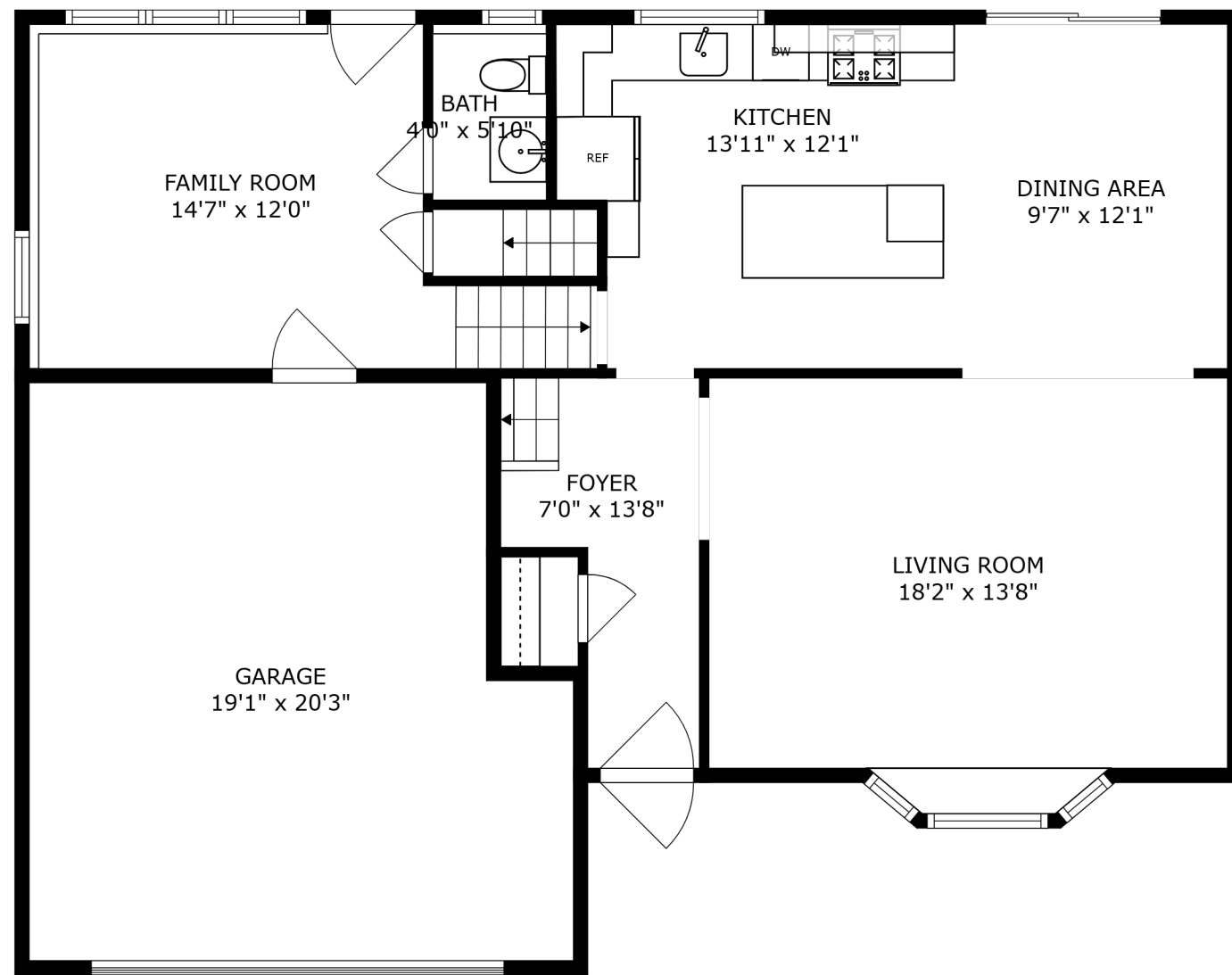
FLOOR 2
