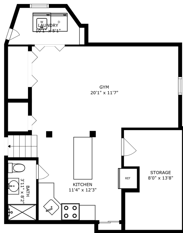
FLOOR 1
