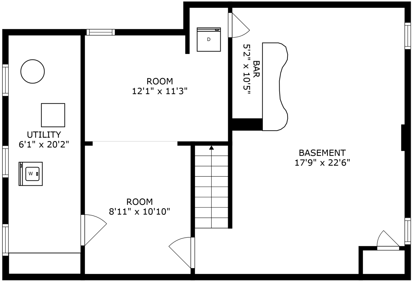
FLOOR 1
