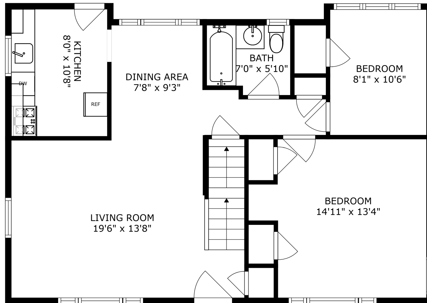
FLOOR 1
