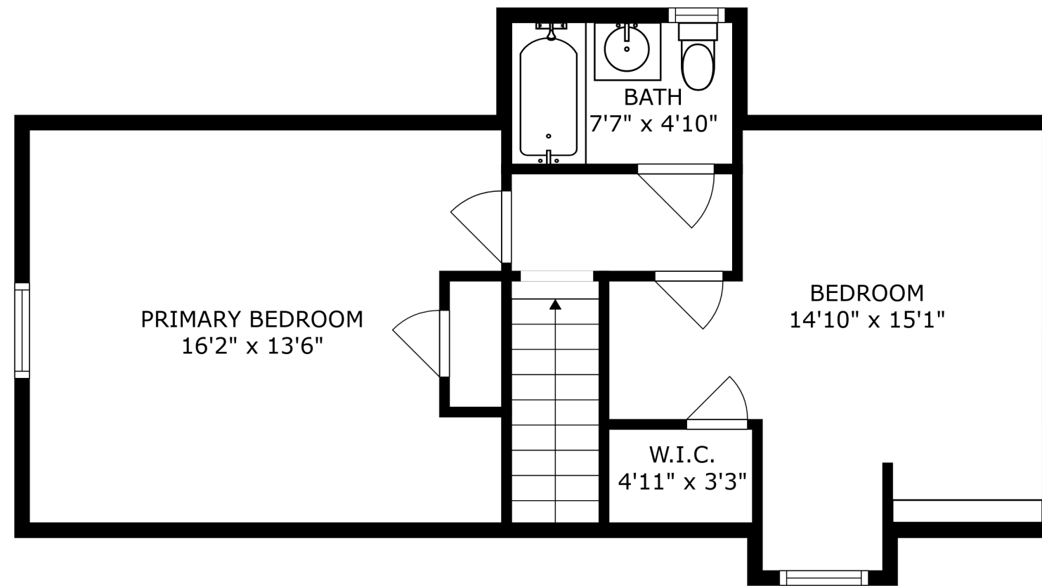
FLOOR 2
