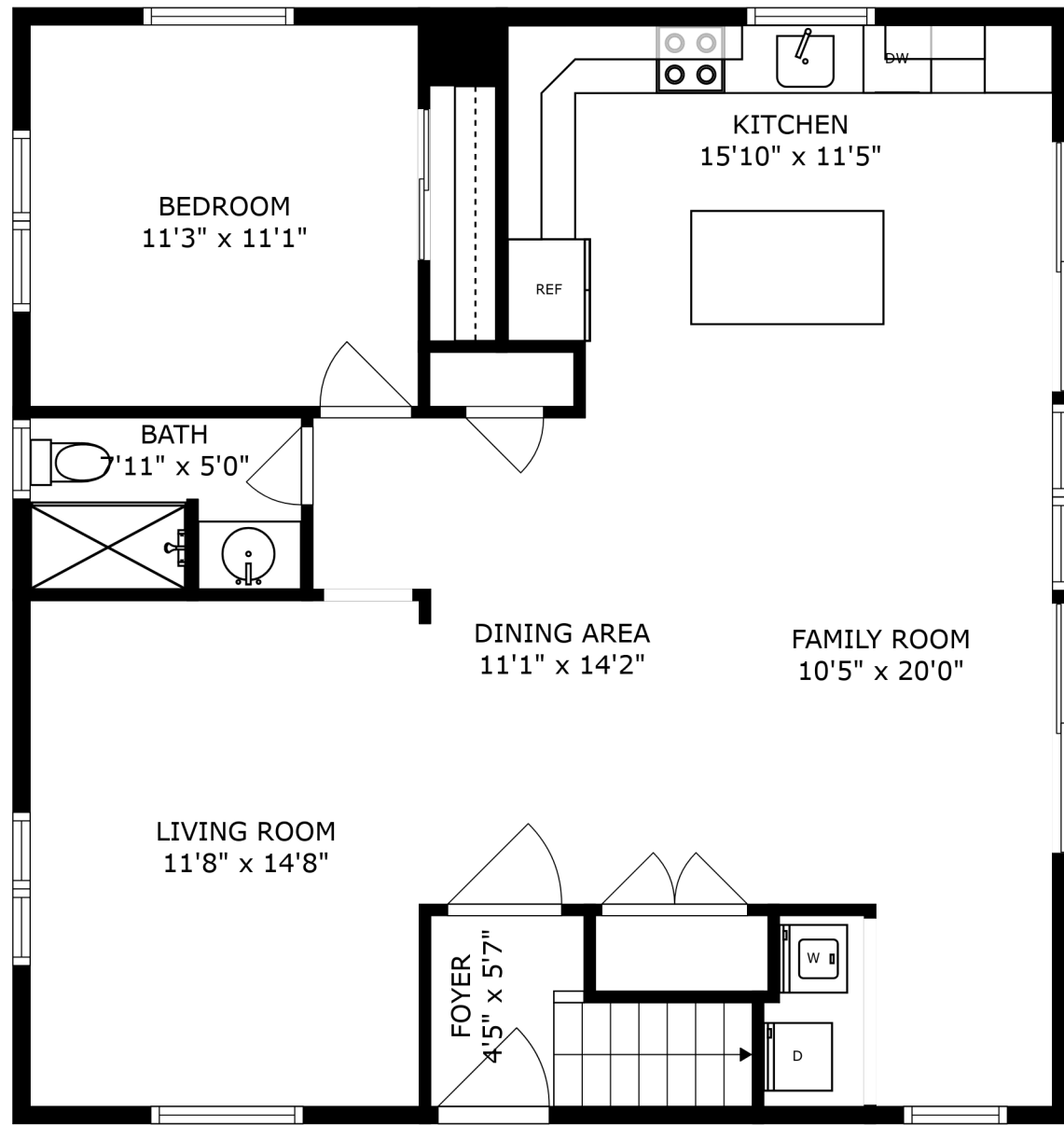
FLOOR 1
