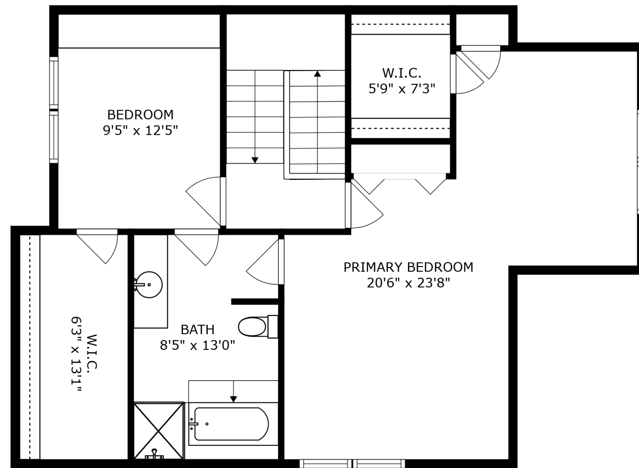
FLOOR 2
