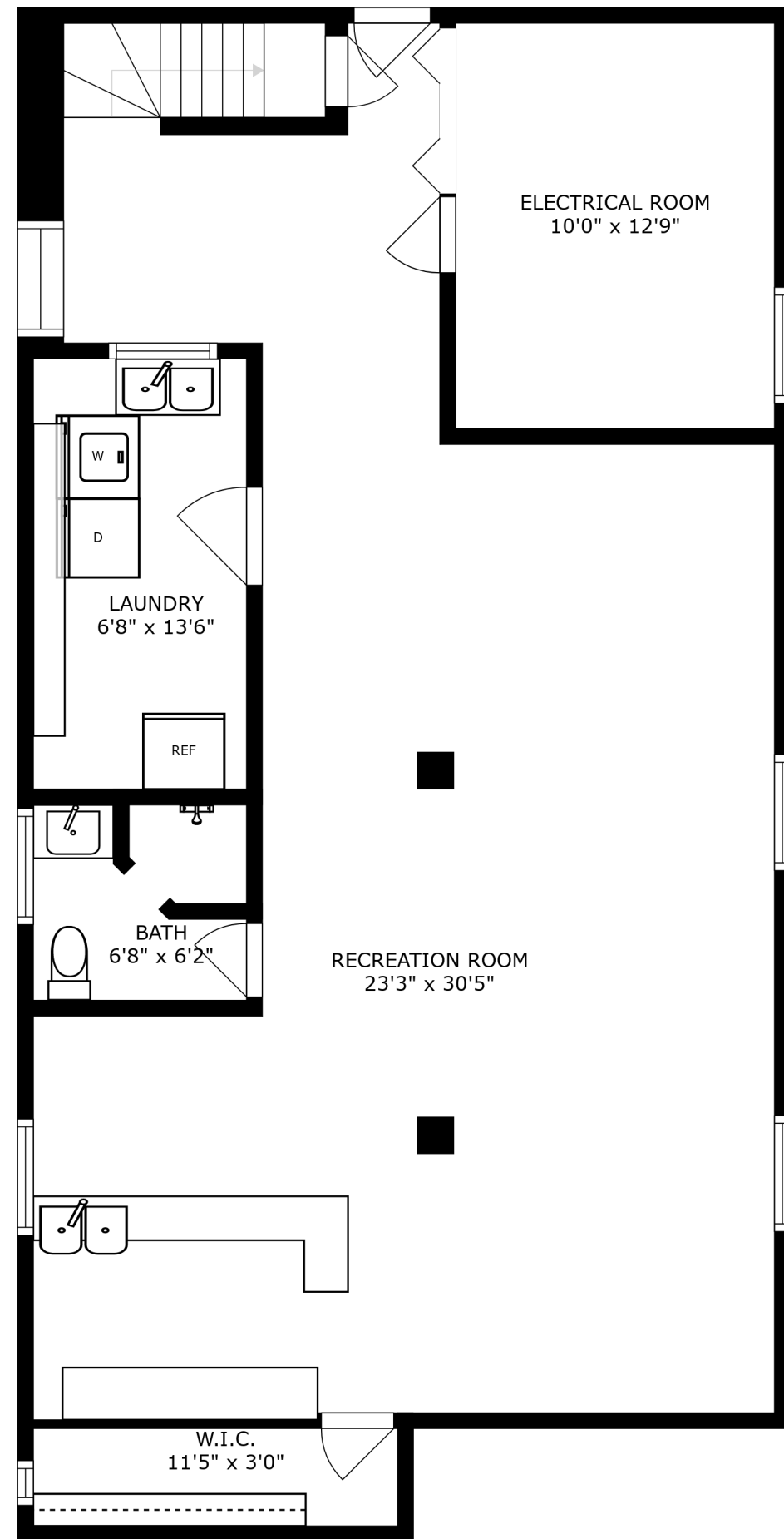
FLOOR 1
