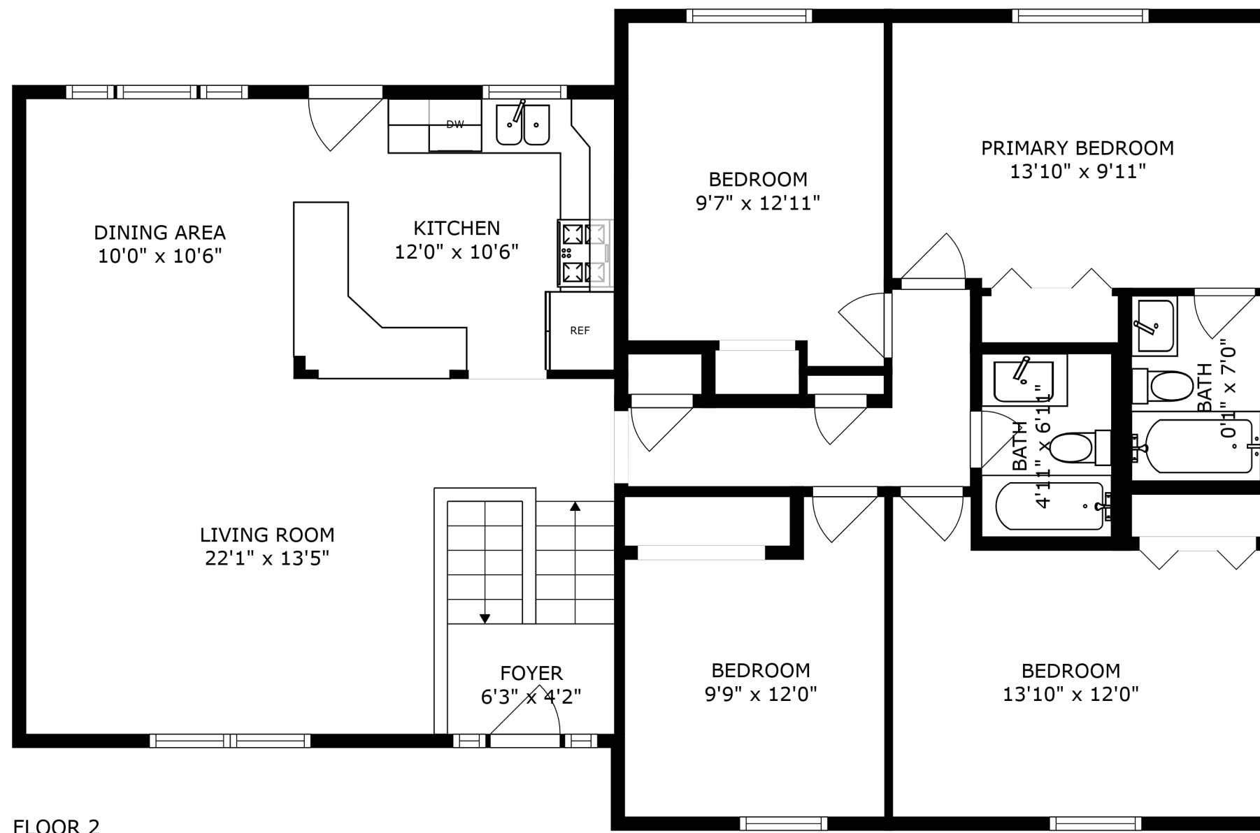
FLOOR 2
