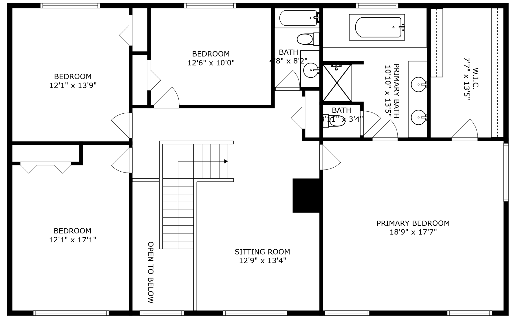
FLOOR 3
