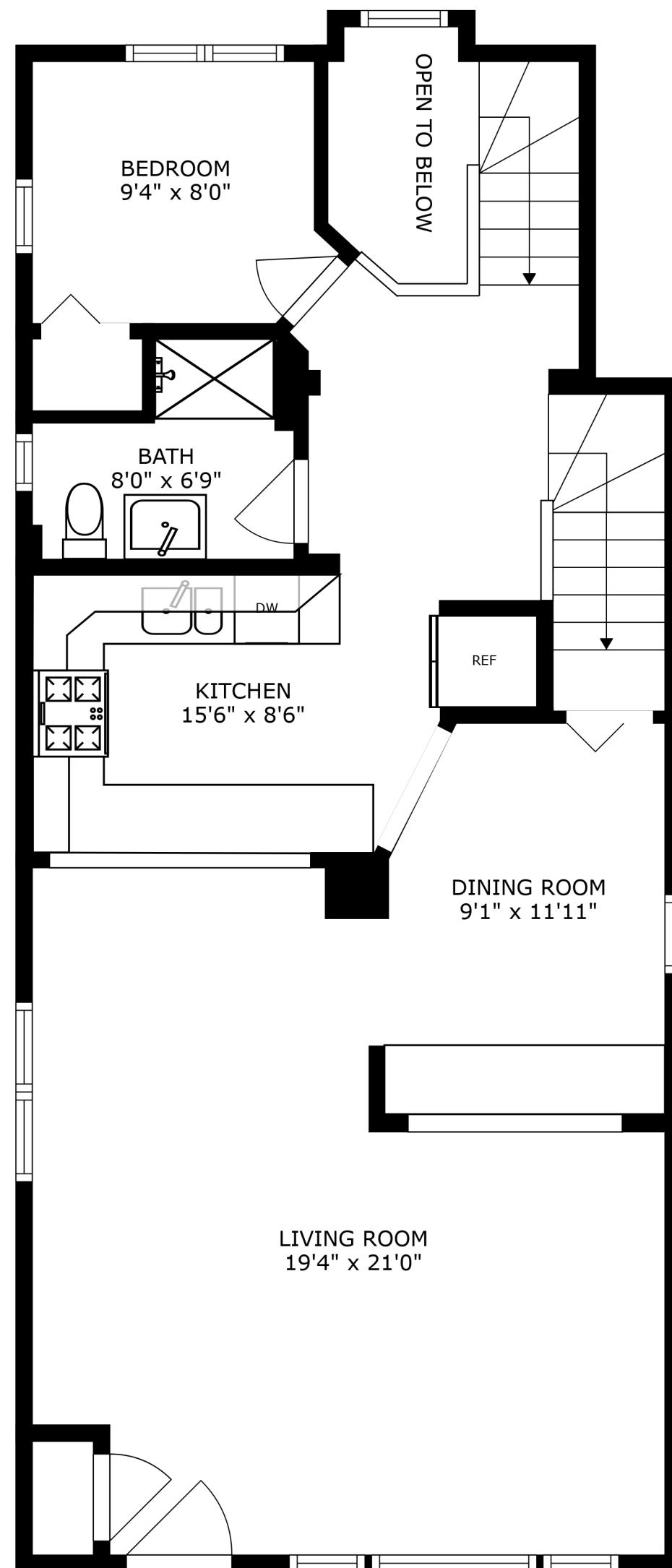
FLOOR 2
