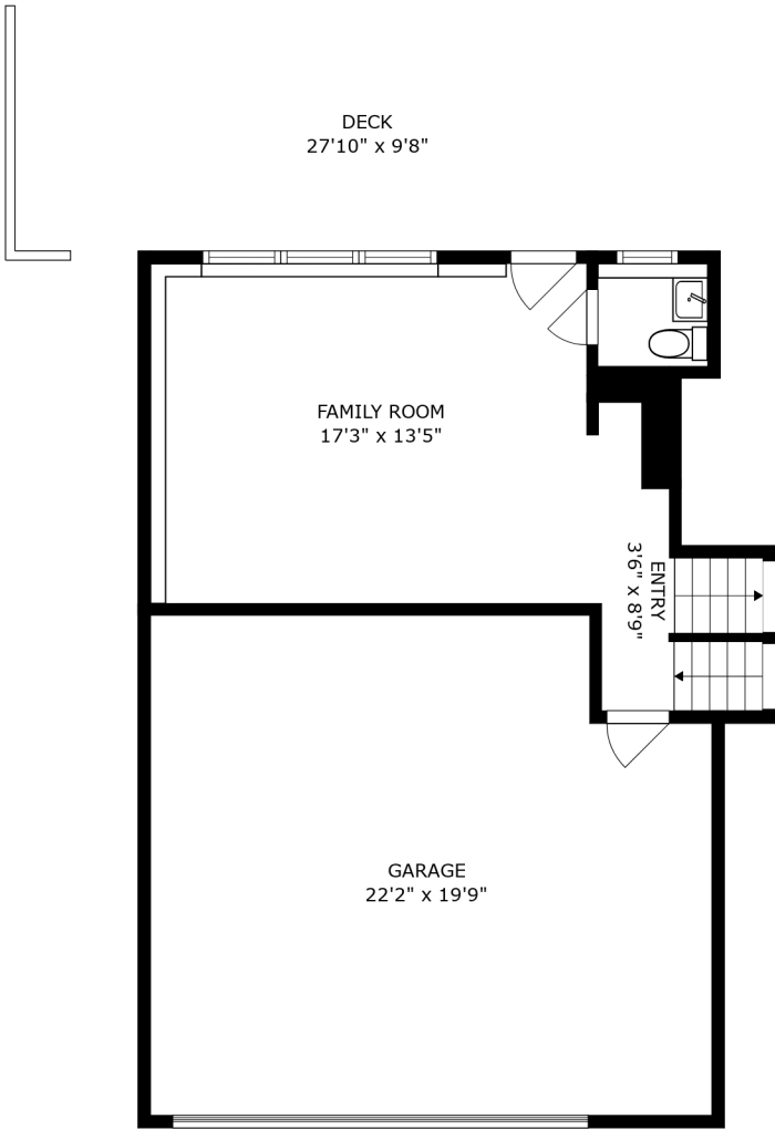
FLOOR 2
