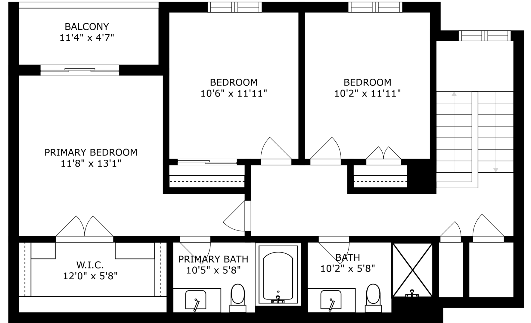
FLOOR 2
