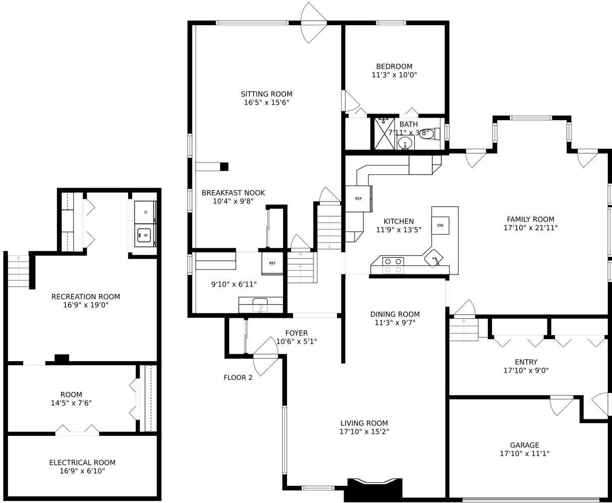
FLOOR 1
