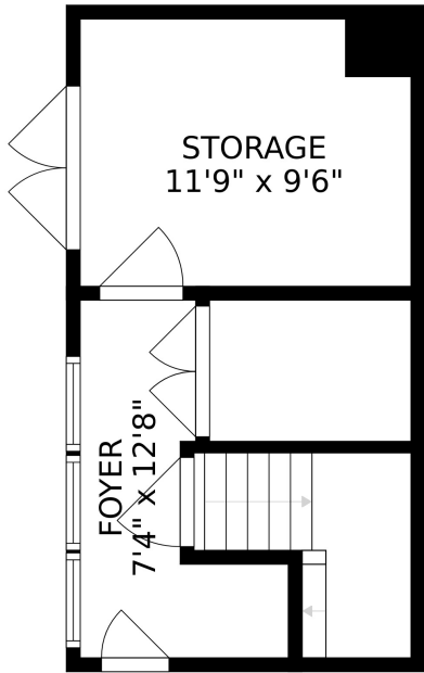
FLOOR 1
