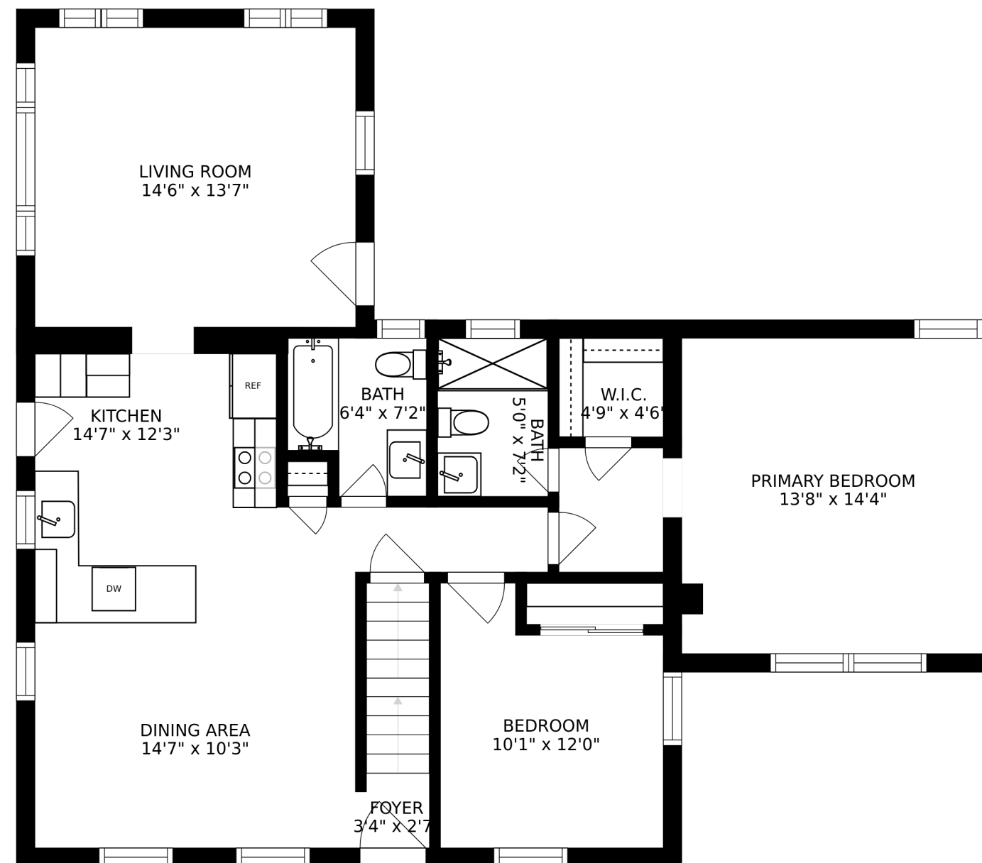
FLOOR 2
