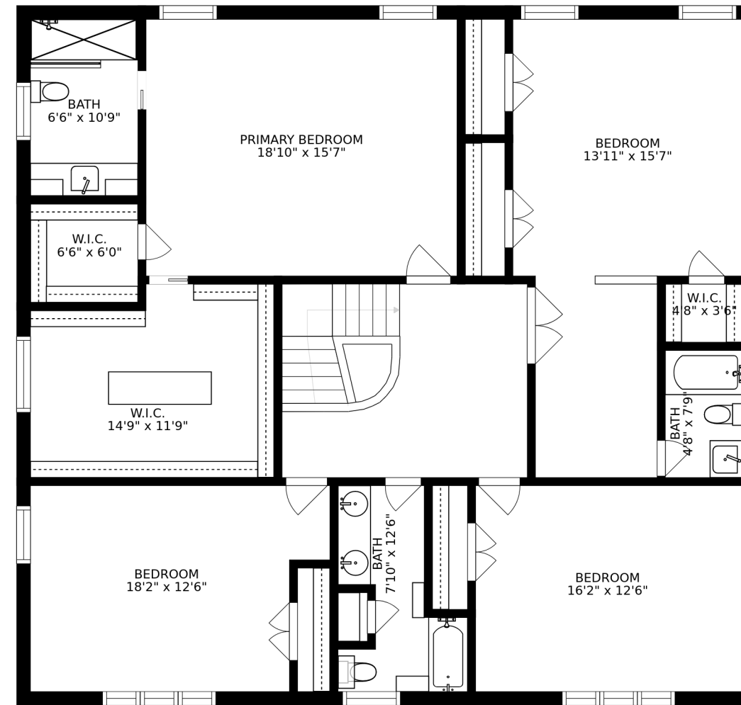
FLOOR 3
