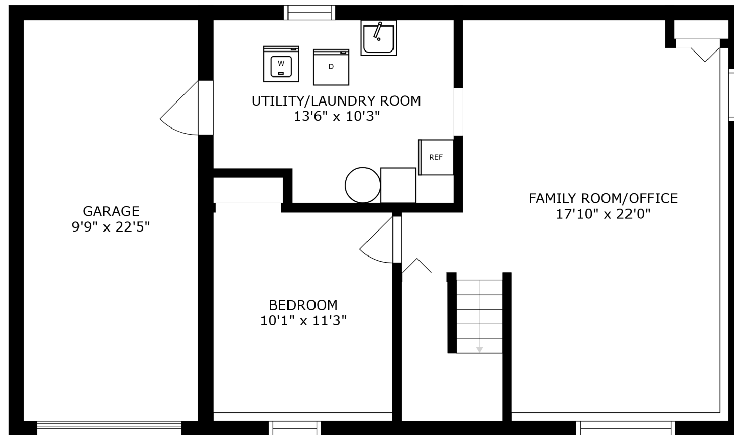
FLOOR 1
