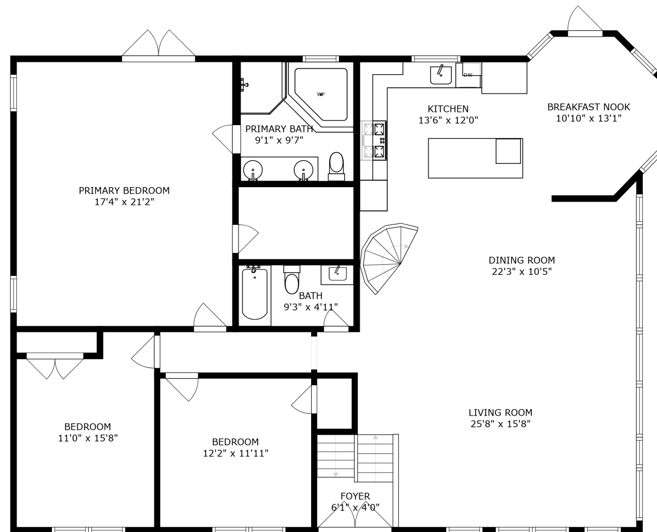
FLOOR 2
