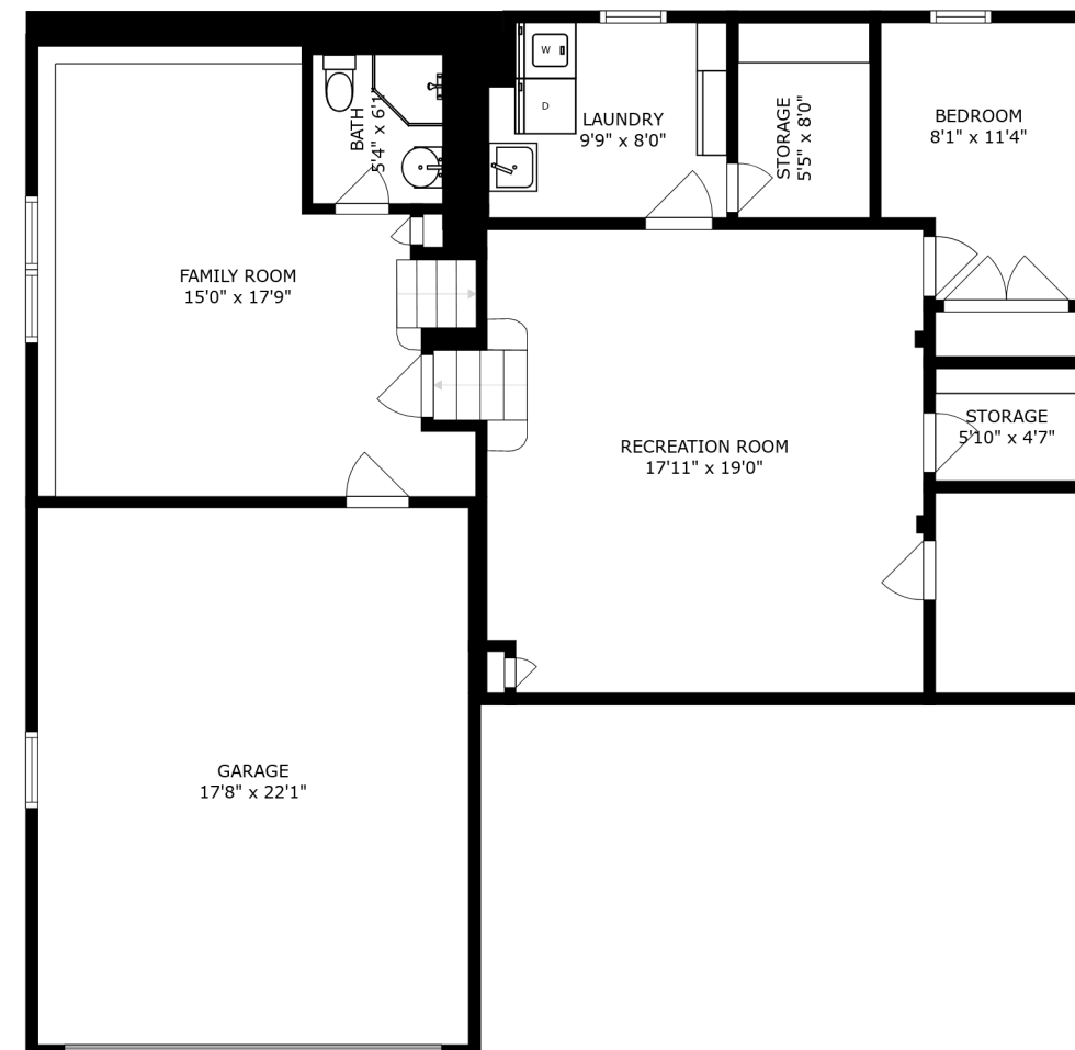
FLOOR 1
