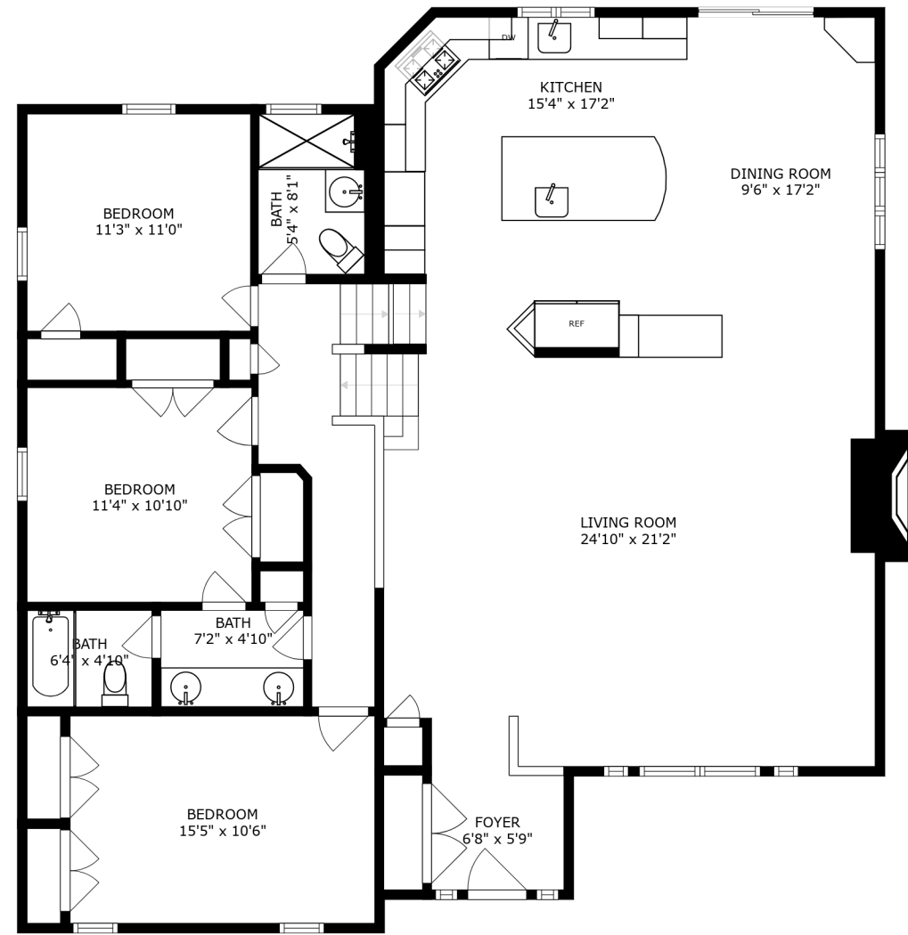
FLOOR 2
