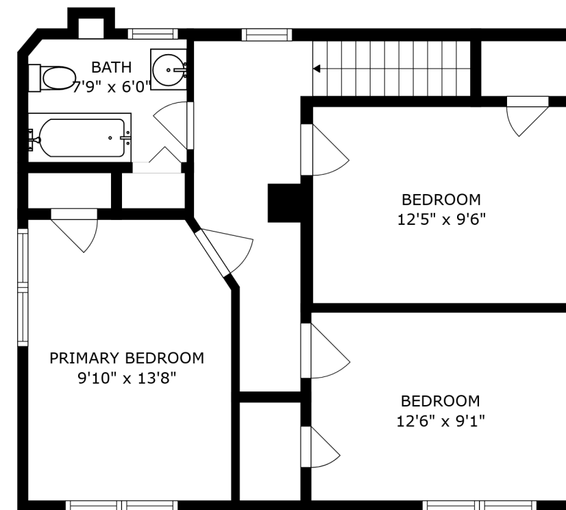
FLOOR 3
