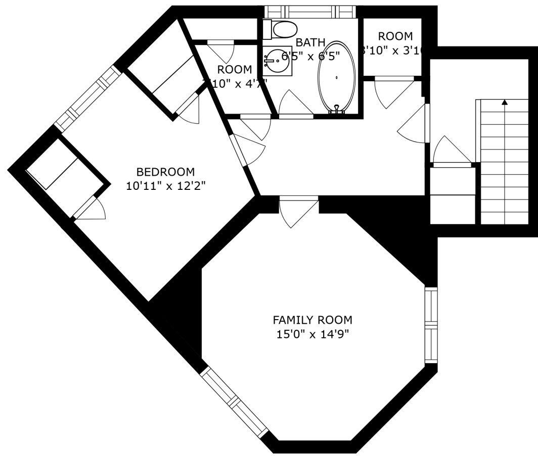
FLOOR 4
