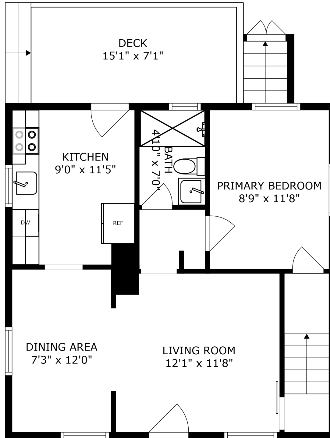
FLOOR 2
