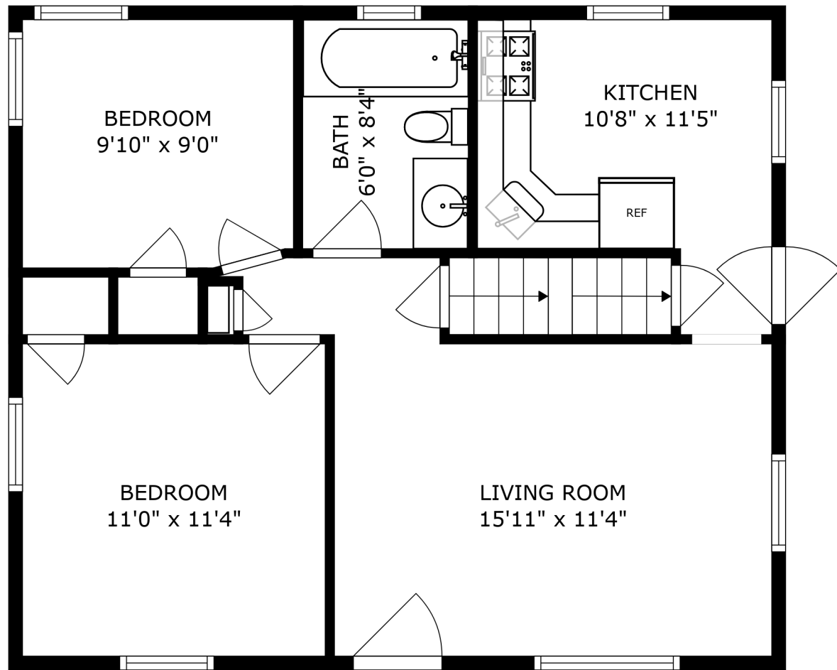
FLOOR 2
