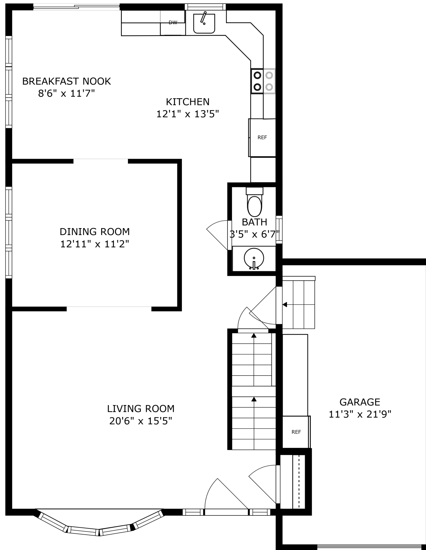
FLOOR 2
