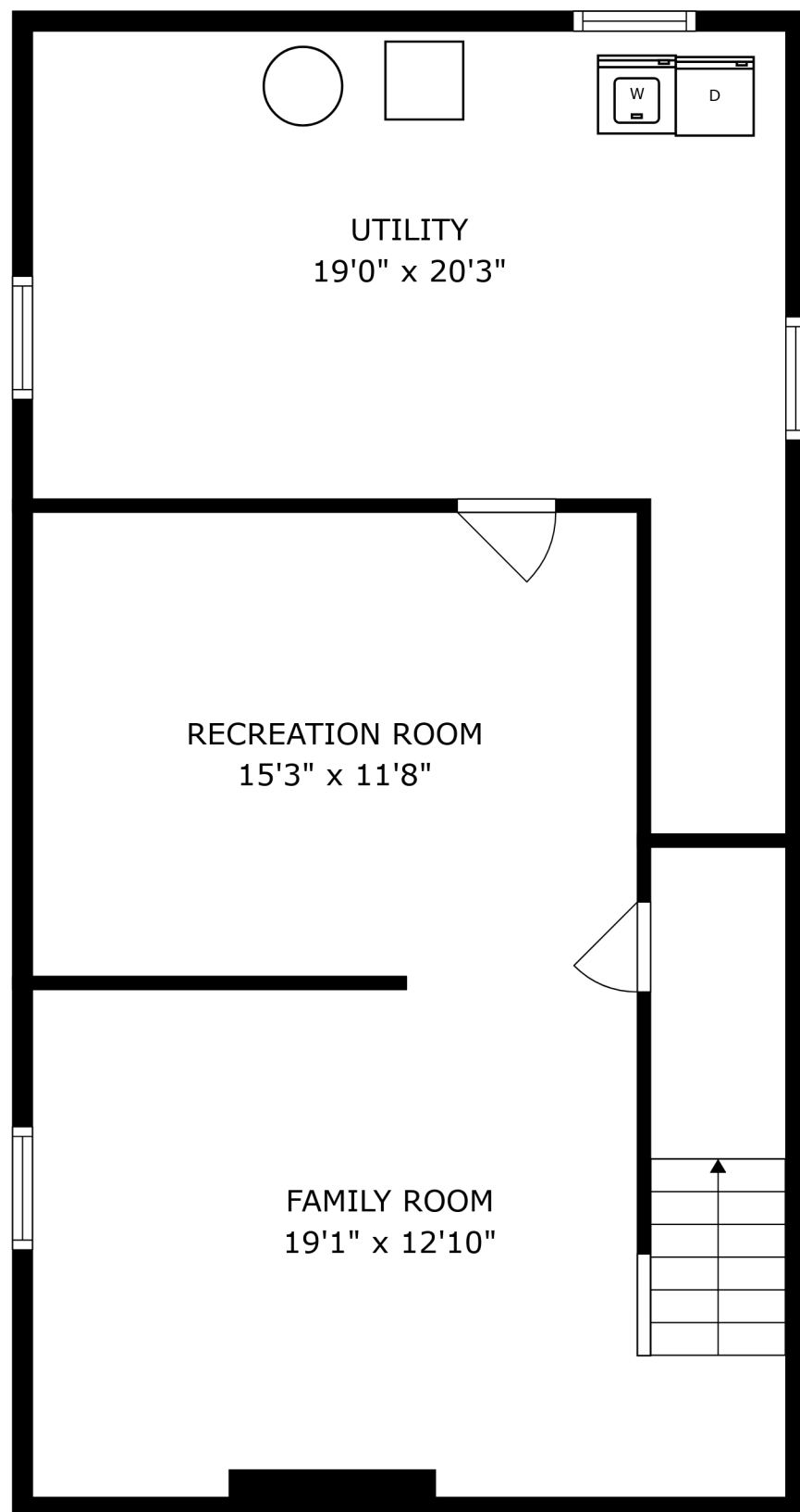
FLOOR 1
