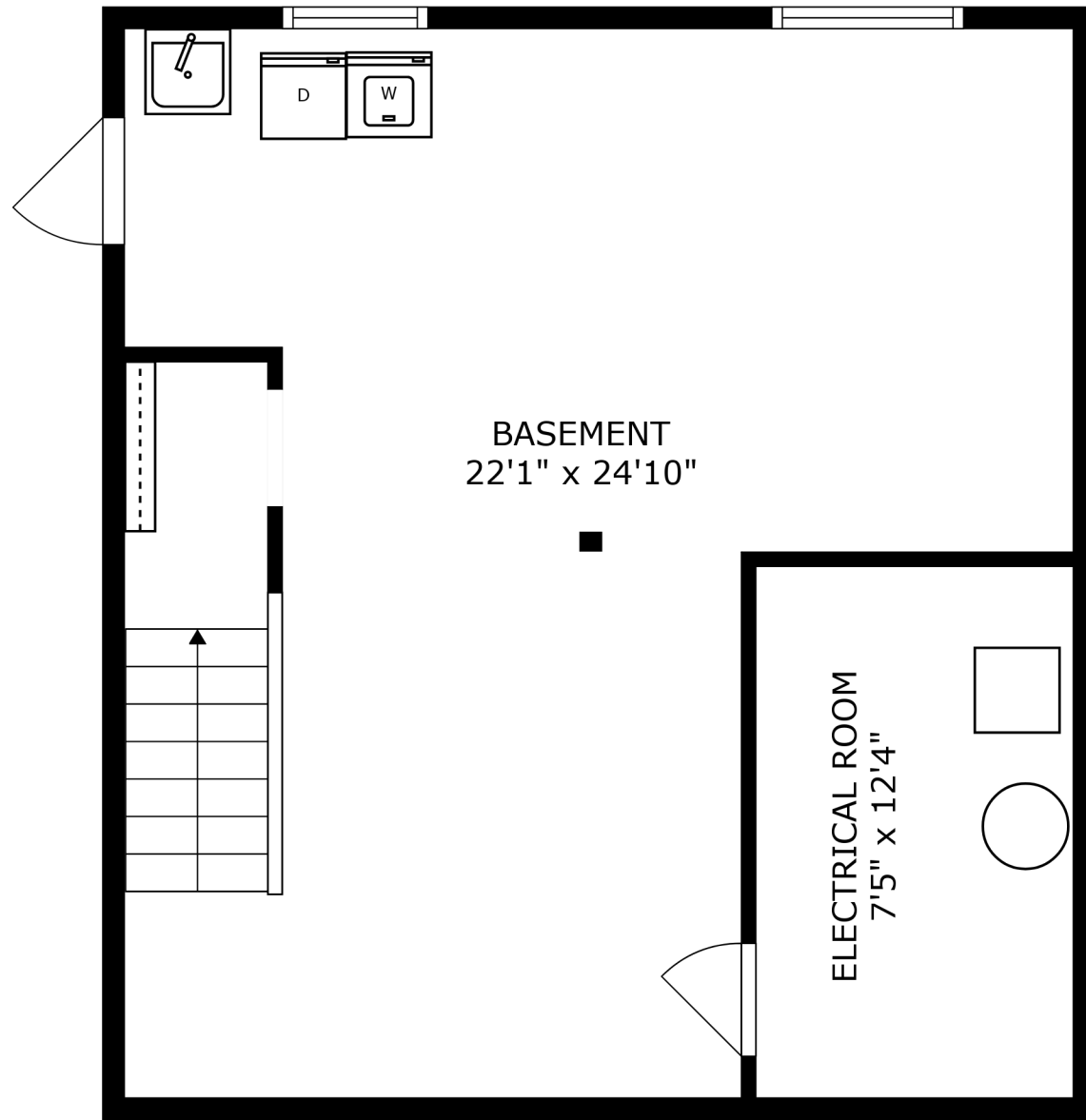
FLOOR 1
