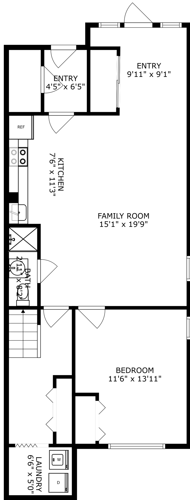
FLOOR 1
