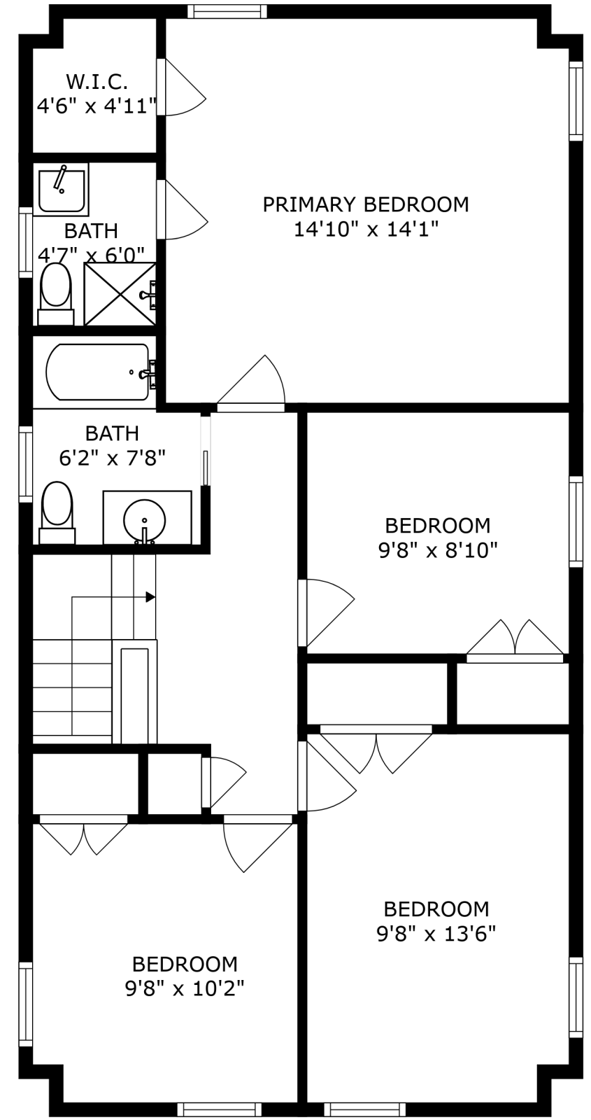
FLOOR 3
