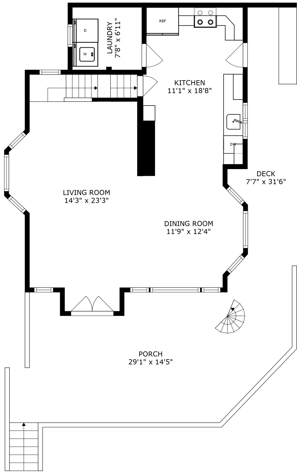
FLOOR 2
