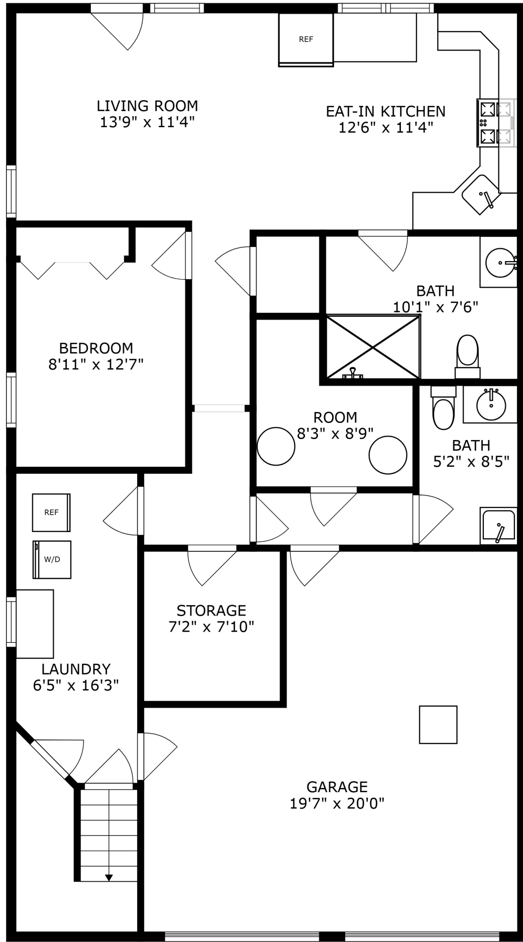
FLOOR 1
