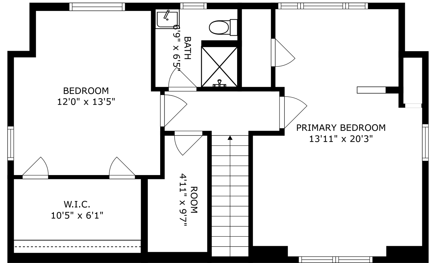
FLOOR 2
