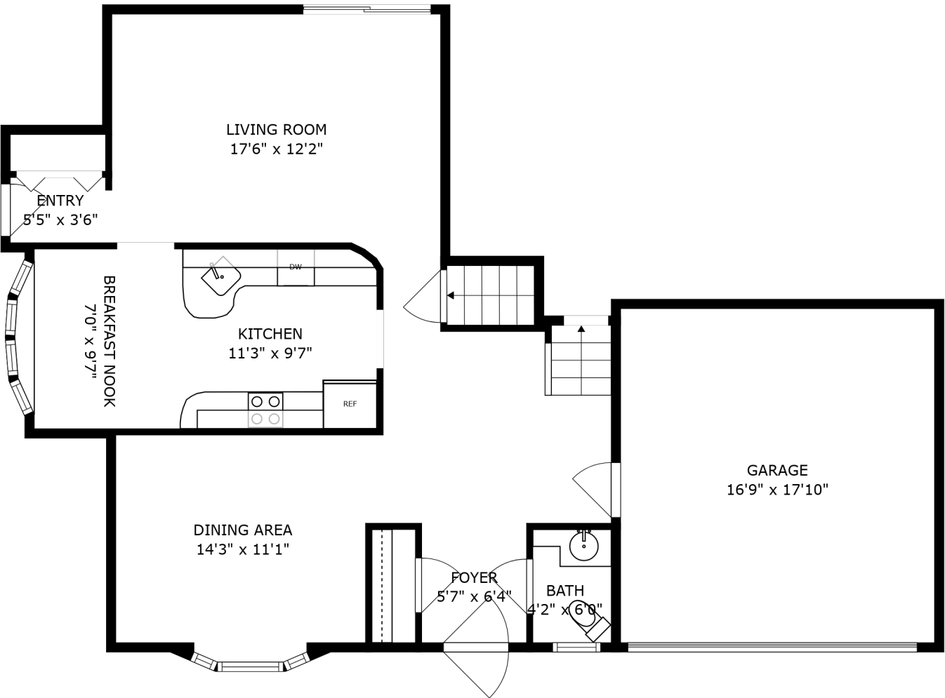
FLOOR 3
